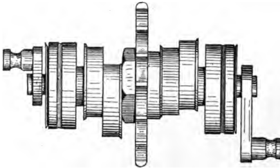
FIG. 368.—Crank Shaft of the "Locomobile" Steam Carriage, showing the cranks at both ends, the ball bearings and eccentrics, and the sprocket at the centre. Most steam carriage engines have similarly arranged crank shafts, although with several makes the entire mechanism is turned from one solid casting.
